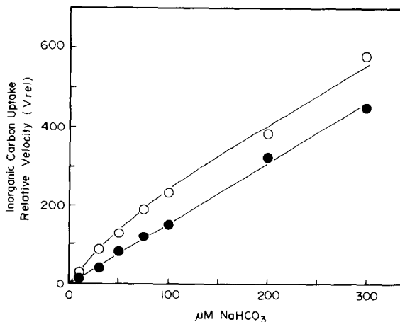
Fig.2. Relative velocities of the initial rate of inorganic carbon uptake in C. reinhardtii as a function of external \text{NaHCO}_3 concentration (pH 7.0) in the absence ( \circ ) or presence ( \bullet ) of 5 \mu\text{M} FCCP. Each point represents the mean value of 4 replicates.
